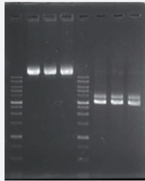
Agarose gel electrophoresis of DNA stained with DNA-Dye NonTox. DNA marker (M) and samples (1-6) were stained with DNA-Dye NonTox, separated by agarose gel electrophoresis and subsequently detected under UV light.
